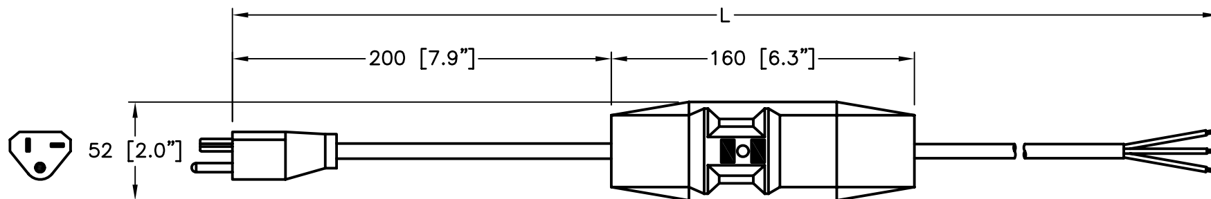
Nema 5-20P
